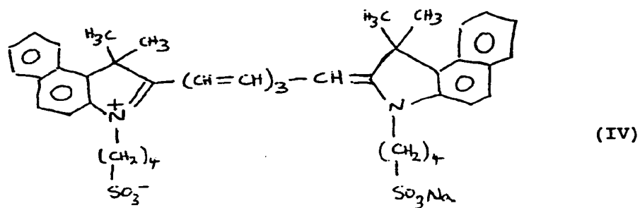
Indocyanine Green (ICG)
